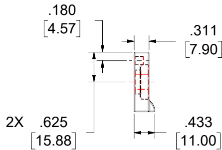
Snubber Receiver
