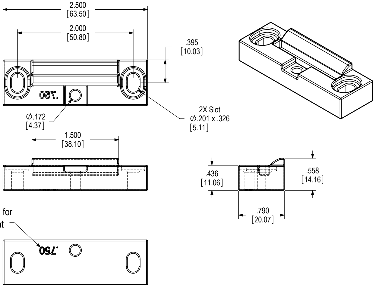
617-715 Snubber Receiver
